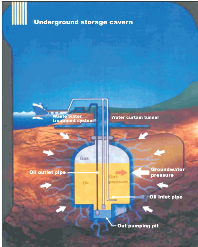
Fig. 1: 3 Dimensional Model Of A Typical Unlined Underground Cavern
