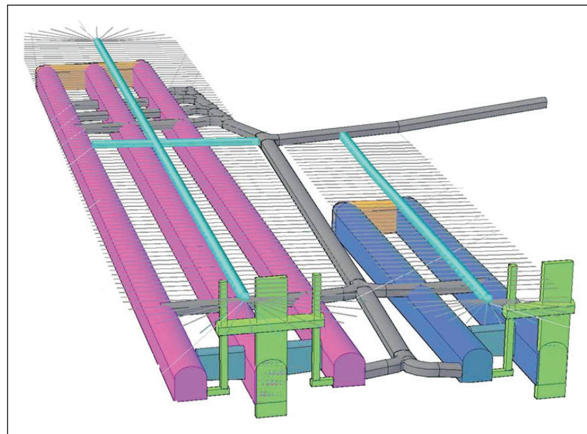
Fig. 2: A Typical Cavern Layout Along With Superimposed Water Curtain System.
